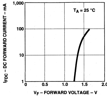
Figure 2a. DC Forward Current vs. Forward Voltage.
