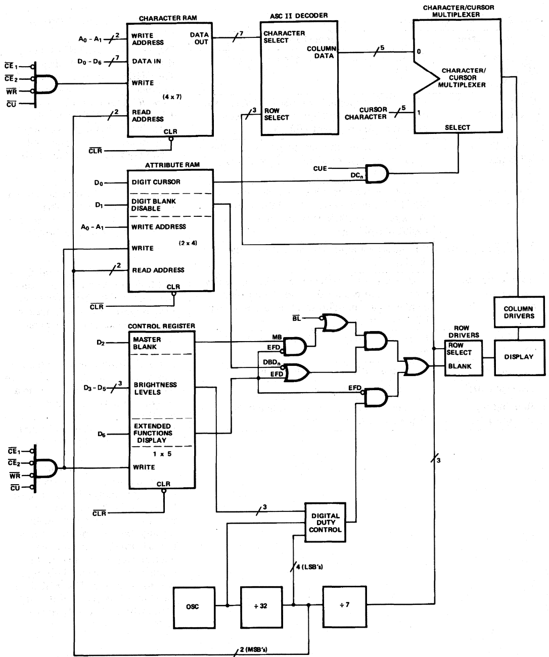
Figure 1. Internal Block Diagram
