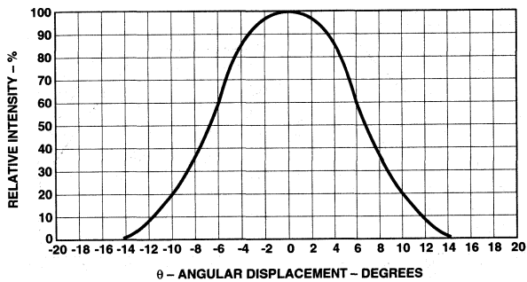
Figure 7. Spatial Radiation Pattern for 15° Viewing Angle Lamps.
