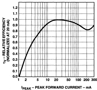
Figure 5. Relative Efficiency vs. Peak Forward Current.
