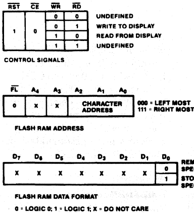
Figure 5. Logic Levels to Access the Flash RAM.
