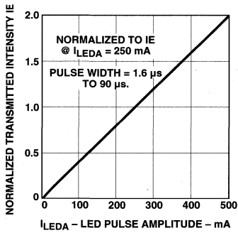
Figure 4. Transmitted Intensity vs. LED Pulse Amplitude.
