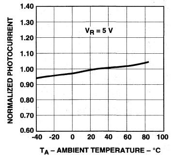
Figure 13. Relative Reverse Light Current vs. Ambient Temperature.
