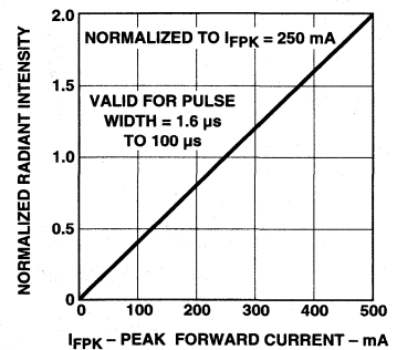
Figure 3b. Normalized Radiant Intensity vs. Peak Forward Current.
