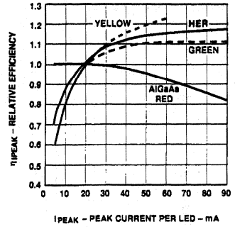
Figure 4. Relative Efficiency (Luminous Intensity per Unit Current) vs. Peak Current. \eta , (300 mA) for AlGaAs Red = 0.7.
