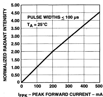
Figure 4. Normalized Radiant Intensity vs. Peak Forward Current.
