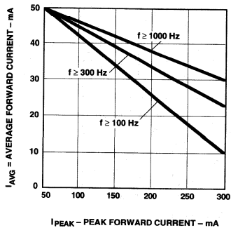
Figure 6. Maximum Average Current vs. Peak Forward Current.
