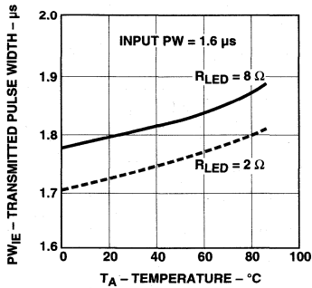
Figure 13. Transmitted Pulse Width vs. Temperature.
