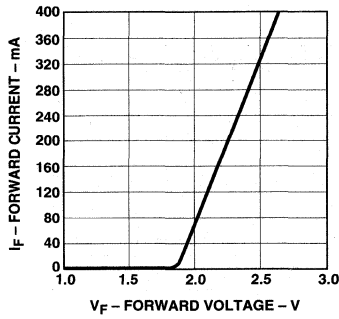
Figure 2a. Forward Current vs. Forward Voltage, HLMA-VL00/VH00.
