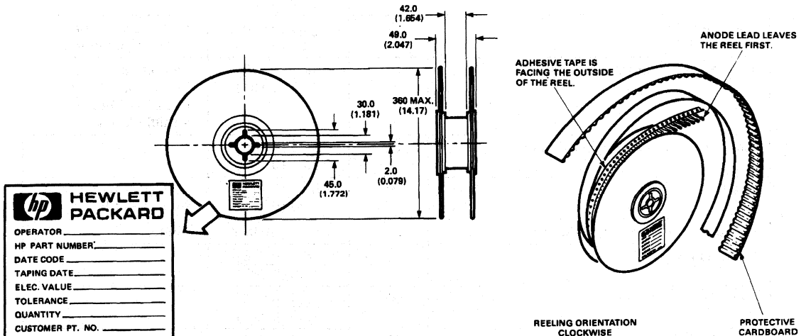
Figure 11. Reel Configuration and Labeling.
