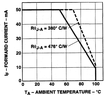
Figure 4. Maximum Forward Current vs. Ambient Temperature for HLMA-/HLMT-QL00/QH00/PL00/PH00. Derating Based on T_{j,MAX} = 110^{\circ}C .
