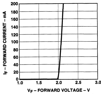
Figure 2a. Forward Current vs. Forward Voltage. HLMA-QL00/QH00/PL00/PH00.
