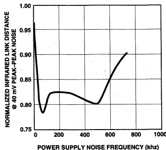
Figure 19b. Infrared Link Distance versus Power Supply Noise Frequency.
