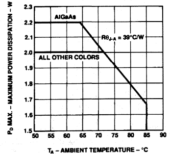
Figure 10. Maximum Allowable Power Dissipation vs. Ambient Temperature. T_j MAX = 150 °C or 120 °C.
