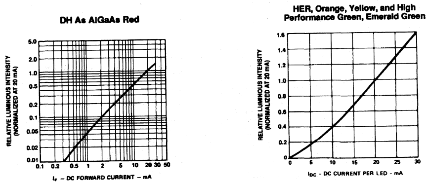
Figure 3. Relative Luminous Intensity vs. Forward Current.
