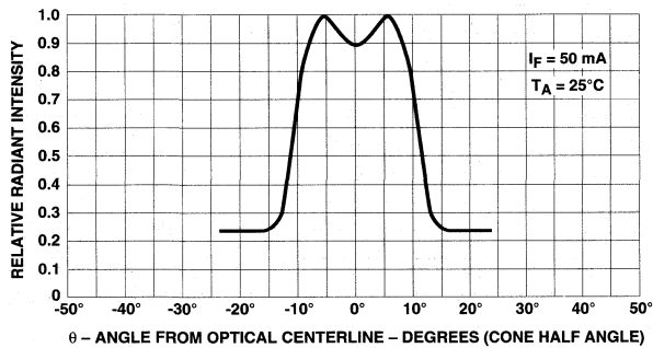
Figure 10. Relative Radiant Intensity vs. Angular Displacement HSDL-4420.
