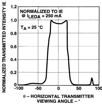
Figure 7. Transmitted Intensity vs. Horizontal Viewing Angle.
