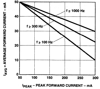
Figure 6. Maximum Average Current vs. Peak Forward Current.
