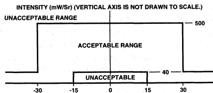
Figure 7. Acceptable Optical Output Intensity Range.
