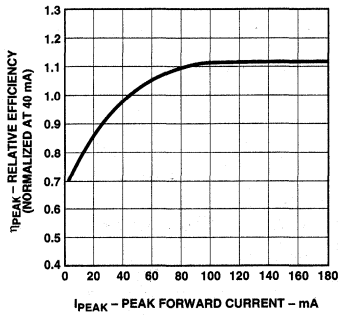
Figure 4c. Relative Efficiency vs. Peak Forward Current, HLMP-V500.
