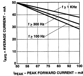
Figure 5b. Maximum Average Current vs. Peak Forward Current for HLMT-QL00/QH00/PL00/PH00.
