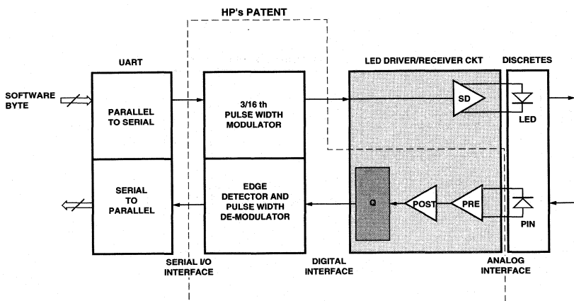
Figure 3. IrDA Physical Layer and HP Patent.
