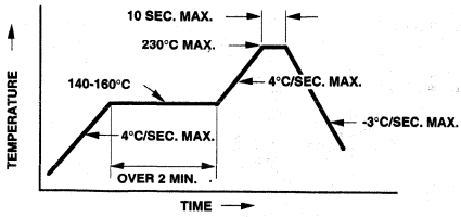
Figure 6. Recommended SMT Reflow Soldering Profile.
