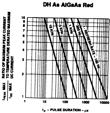
Figure 6. Maximum Tolerable Peak Current vs. Pulse Duration. ( I_{DC, \text{MAX}} as per MAX Ratings).
