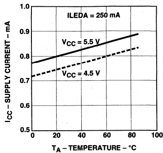
Figure 11. Supply Current vs. Temperature.
