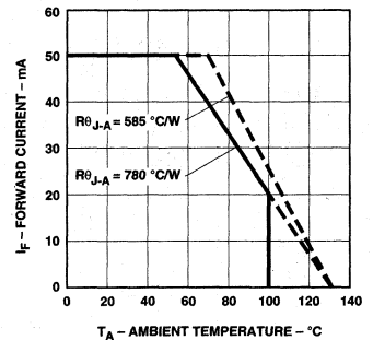
Figure 4a. Maximum DC Current vs. Ambient Temperature for AS T-1 3/4 Lamps. Derating Based on T_{jMAX} = 130^{\circ}C .
