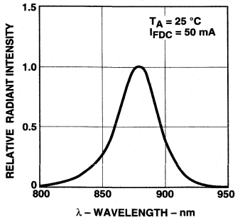
Figure 1. Relative Radiant Intensity vs. Wavelength.
