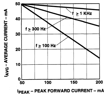
Figure 5a. Maximum Average Current vs. Peak Forward Current for HLMA-QL00/QH00/PL00/PH00.
