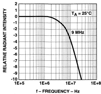
Figure 11. Relative Radiant Intensity vs. Frequency.
