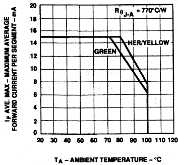
Figure 5. Maximum Allowable Average or DC Current vs. Ambient Temperature.
