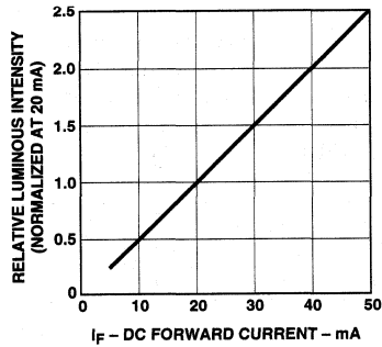
Figure 3a. Relative Luminous Intensity vs. DC Forward Current. HLMA-QL00/QH00/PL00/PH00.
