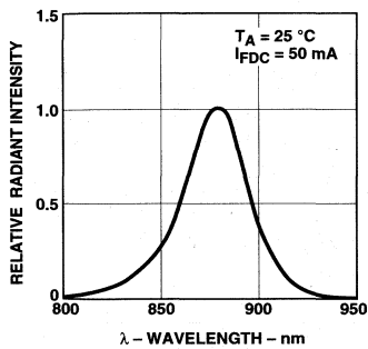
Figure 1. Relative Radiant Intensity vs. Wavelength.
