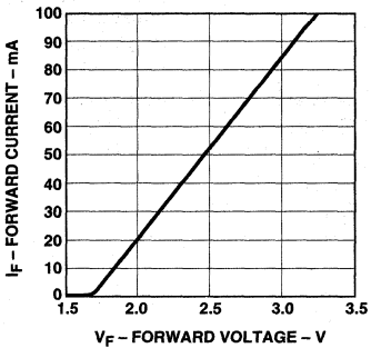
Figure 2b. Forward Current vs. Forward Voltage, TS-AllnGaP.
