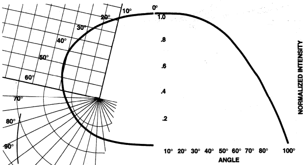
Figure 6. Intensity vs. Angle.
