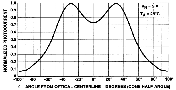
Figure 18. Relative Radiant Intensity vs. Angular Displacement. HSDL-5400.
