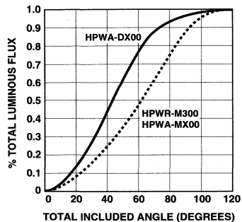
Figure 6a. HPWR-M300/HPWA-XX00 Percent Total Luminous Flux vs. Total Included Angle.
