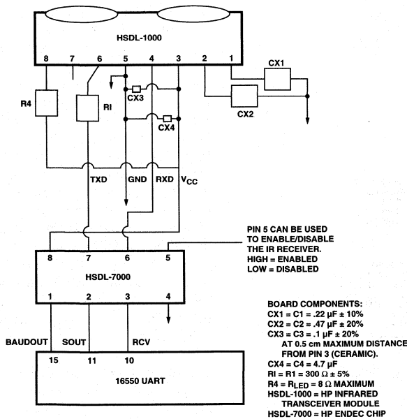
Figure 11. 16550 UART Application Diagram.
