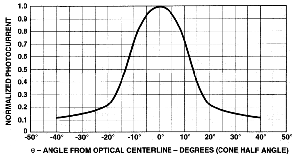
Figure 19. Relative Radiant Intensity vs. Angular Displacement. HSDL-5420.
