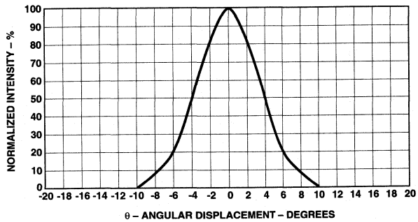
Figure 6. Spatial Radiation Pattern for 8° Viewing Angle Lamps.
