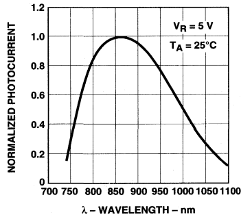
Figure 17. Relative Spectral Sensitivity vs. Wavelength.
