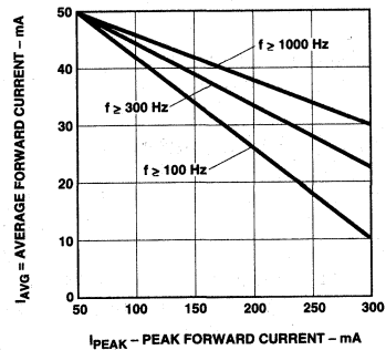
Figure 13. Maximum Average Current vs. Peak Forward Current.
