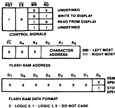
Figure 5. Logic Levels to Access the Flash RAM.
