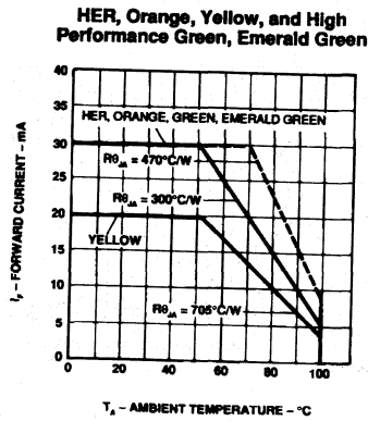
Figure 5. Maximum Forward dc Current vs. Ambient Temperature. Derating Based on T_j, \text{MAX} = 110^\circ\text{C} .
