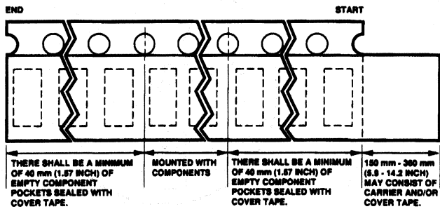
Figure 11. Tape Leader and Trailer Dimensions.
