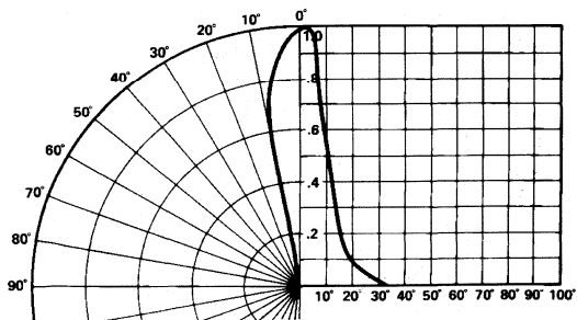
Figure 9. Relative Luminous Intensity vs. Angular Displacement. HLMF-D105.
