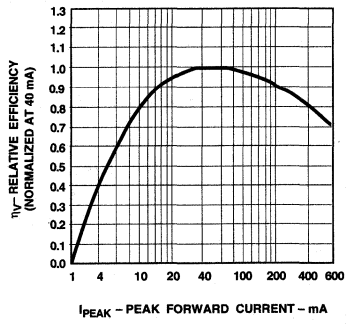
Figure 4b. Relative Efficiency vs. Peak Forward Current, HLMP-V100.
