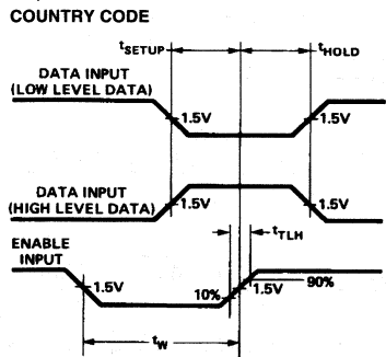
Figure 1. Timing Diagram.
