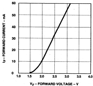
Figure 12. Forward Current vs. Forward Voltage.
