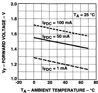
Figure 2c. Forward Voltage vs. Ambient Temperature.
