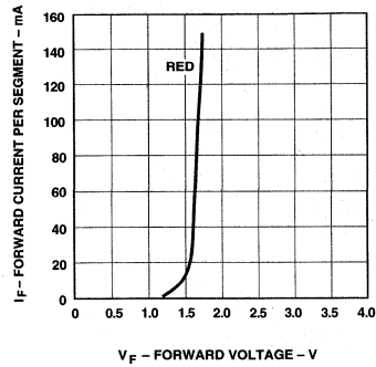
Figure 3. Forward Current vs. Forward Voltage.
