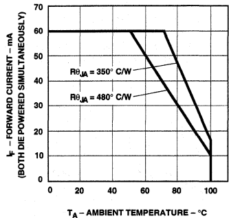
Figure 5a. Maximum Forward DC Current vs. Ambient Temperature, HLMA-VL00/VH00.
