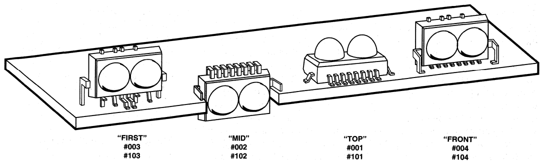
Figure 15. HSDL-1000 Mounting Options.
