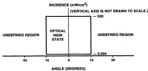
Figure 8. Optical High State Acceptable Range.
