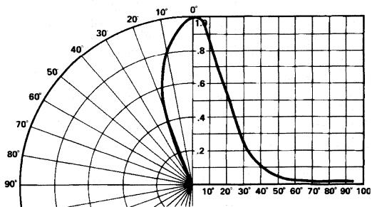
Figure 10. Relative Luminous Intensity vs. Angular Displacement. HLMF-K105.
