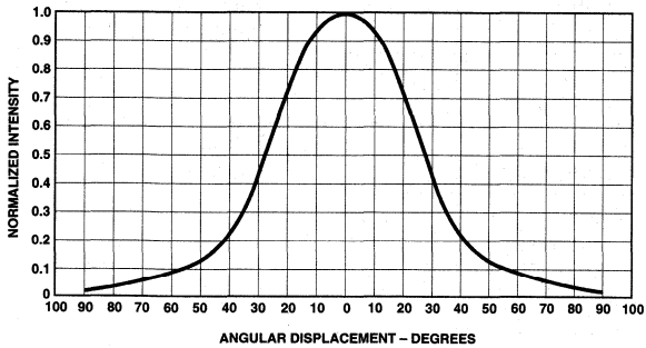
Figure 8. Normalized Luminous Intensity vs. Angular Displacement. HLMP-J100/J150.
