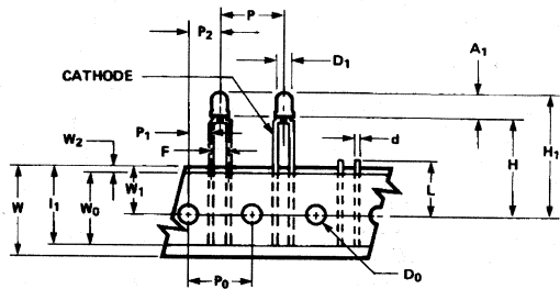
Figure 2. T-1 High Profile Lamps, Option 002.
