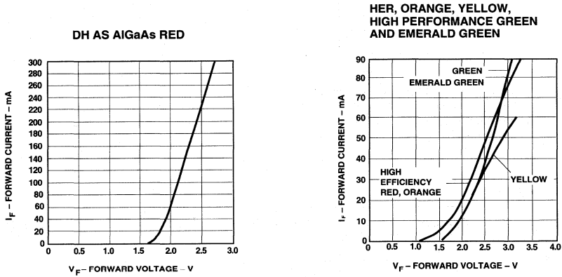
Figure 2. Forward Current vs. Forward Voltage.
