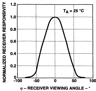
Figure 10. Receiver Responsivity vs. Viewing Angle.
