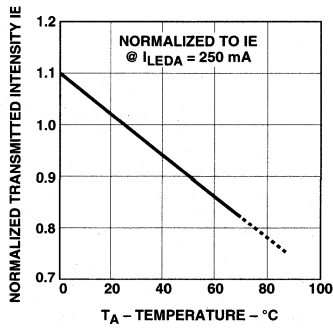
Figure 5. Transmitted Intensity vs. Temperature.
