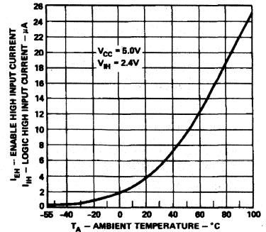
Figure 8. Typical Logic and Enable High Input Current vs. Ambient Temperature.
