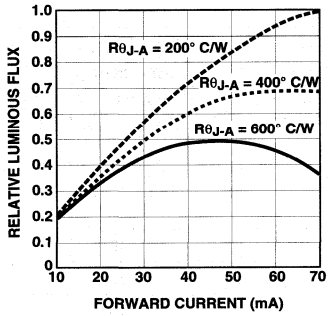
Figure 3a. HPWR-M300 Relative Luminous Flux vs. Forward Current.
