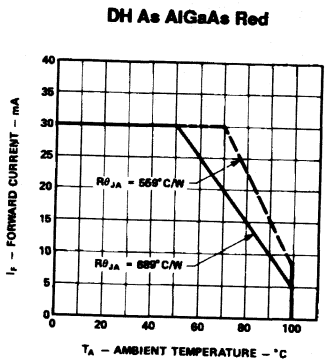
Figure 5. Maximum Forward dc Current vs. Ambient Temperature. Derating Based on T_j, \text{MAX} = 110^\circ\text{C} .
