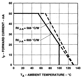
Figure 4b. Maximum DC Current vs. Ambient Temperature for TS T-1 3/4 Lamps. Derating Based on T_{jMAX} = 130^{\circ}C .
