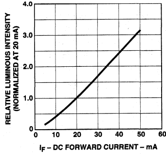
Figure 3b. Relative Luminous Intensity vs. DC Forward Current. HLMT-QL00/QH00/PL00/PH00.
