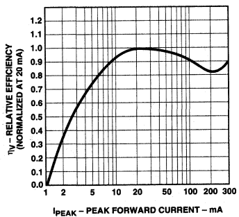
Figure 11. Relative Efficiency vs. Peak Forward Current.
