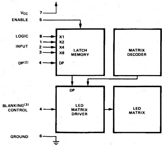
Figure 2. Block Diagram.
