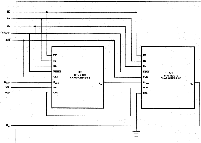
Figure 3. Cascaded ICs.
