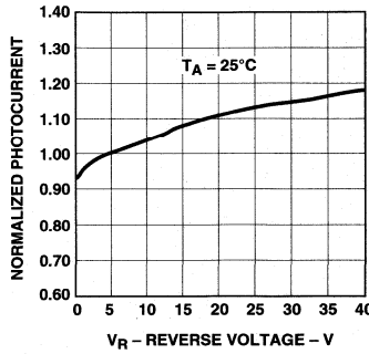
Figure 15. Reverse Light Current vs. Reverse Voltage.
