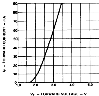
Figure 17. Forward Current vs. Forward Voltage.
