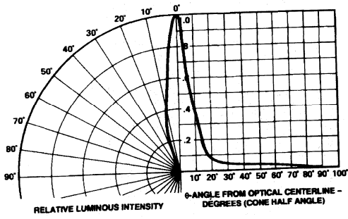
Figure 7. Relative Luminous Intensity vs. Angular Displacement. HLMP-8115/-8X05.
