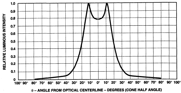
Figure 10. Relative Luminous Intensity vs. Angular Displacement. HLMP-C110.
