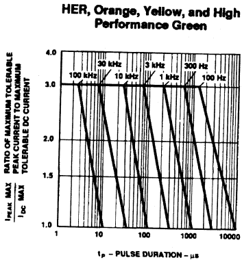
Figure 6. Maximum Tolerable Peak Current vs. Pulse Duration. ( I_{DC, \text{MAX}} as per MAX Ratings).
