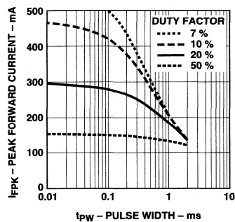
Figure 7. Maximum Peak Forward Current vs. Duty Factor.
