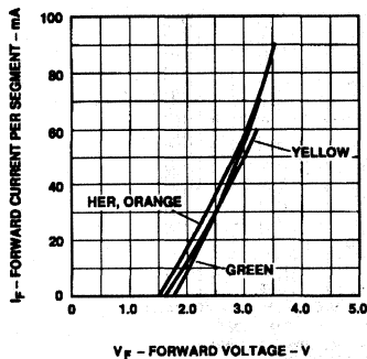
Figure 11. Forward Current vs. Forward Voltage Characteristics.
