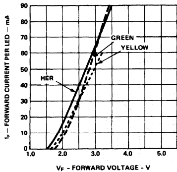
Figure 9. Forward Current vs. Forward Voltage Characteristics.
