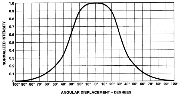
Figure 6. Spatial Radiation Pattern for HLMA-DL05/DH05 65° Lamps.
