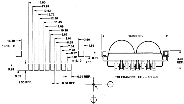
Figure 16d. Pad Layout Diagram Option #X04.
