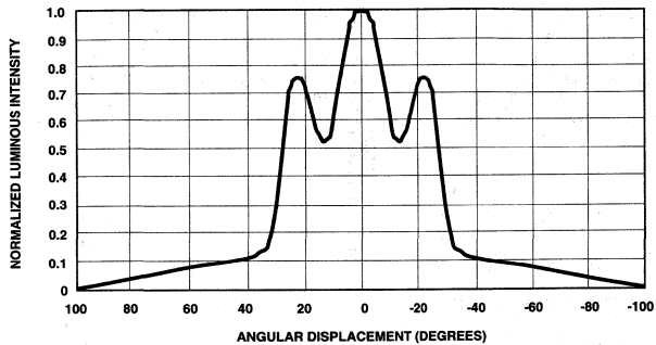
Figure 8a. Relative Intensity vs. Angle, HLMP-V100 Horizontal Axis.
