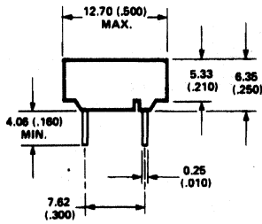
END VIEW
