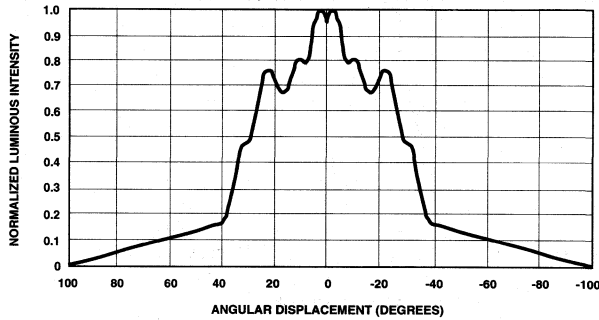
Figure 7a. Relative Intensity vs. Angle, HLMA-VL00/VH00 Horizontal Axis.
