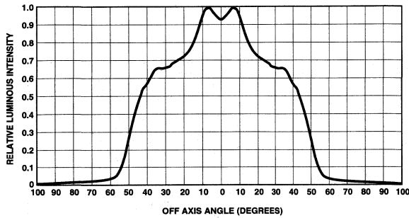
Figure 5a. HPWR-M300, HPWA-MX00 Relative Luminous Intensity vs. Off Axis Angle.
