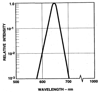
Figure 8. Relative Intensity vs. Wavelength.
