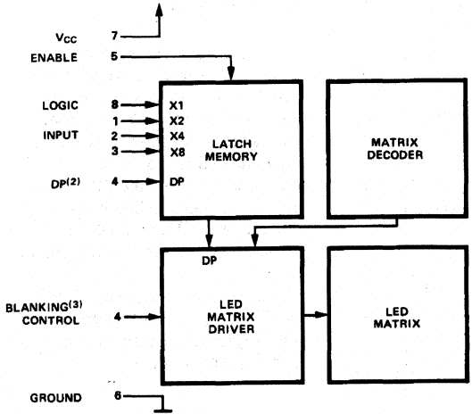
Figure 2. Logic Block Diagram.
