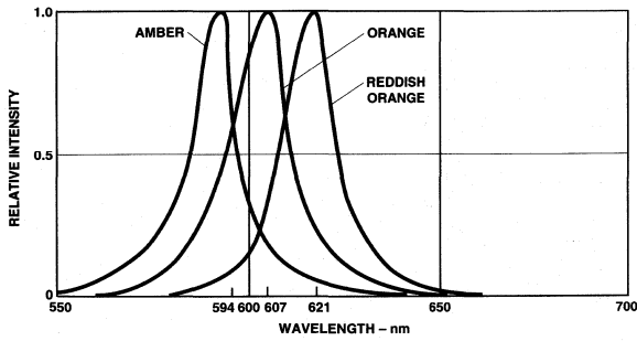
Figure 1. Relative Intensity vs. Wavelength.
