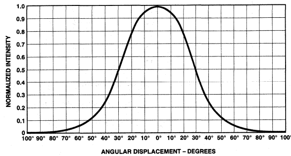
Figure 7. Spatial Radiation Pattern for HLMA-KL05/KH05 60° Lamps.
