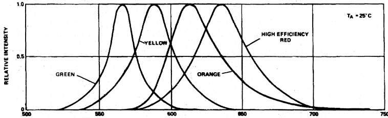
Figure 1. Relative Intensity vs. Wavelength.
