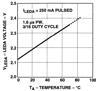
Figure 2. LED Voltage vs. Temperature.
