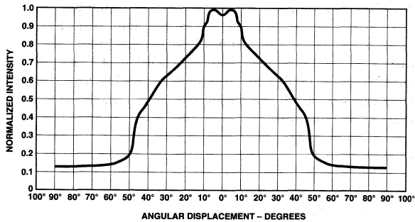
Figure 10. HLMP-P106/-P156.
