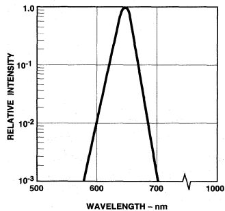
Figure 1. Relative Intensity vs. Wavelength.
