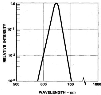
Figure 2. Relative Intensity vs. Wavelength.
