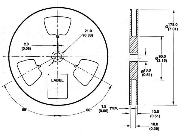
Figure 9. Reel Dimensions.
