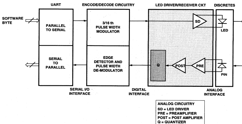
Figure 6. IrDA Physical Layer Block Diagram.
