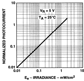
Figure 14. Reverse Light Current vs. Irradiance
