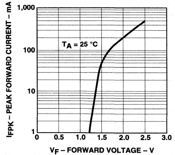
Figure 2b. Peak Forward Current vs. Forward Voltage.
