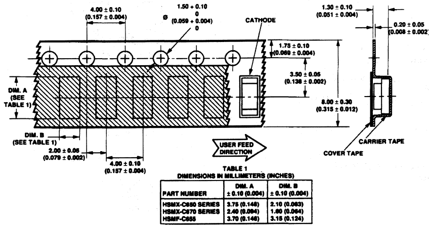
Figure 10. Tape Dimensions.
