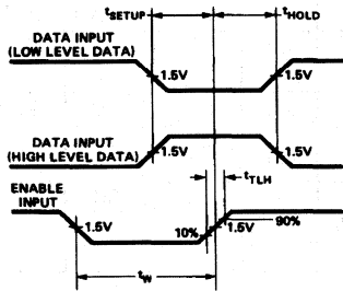
Figure 1. Timing Diagram of 5082-7300 Series Logic.
