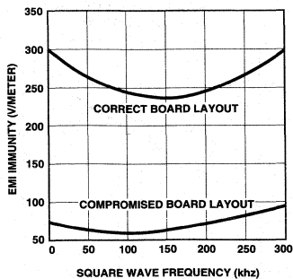
Figure 19a. EMI Immunity vs. Square Wave Noise Signal Frequency.
