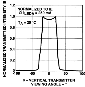
Figure 8. Transmitted Intensity vs. Vertical Viewing Angle.
