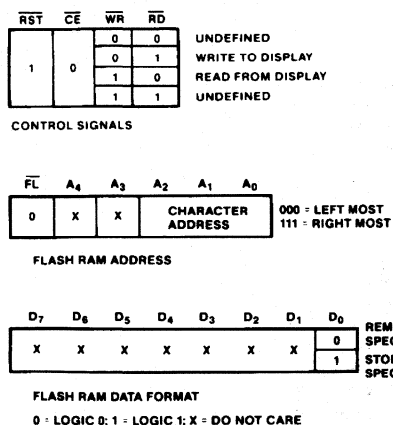
Figure 5. Logic Levels to Access the Flash RAM.
