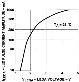
Figure 1. LED Pulse Current Amplitude vs. LED Voltage.
