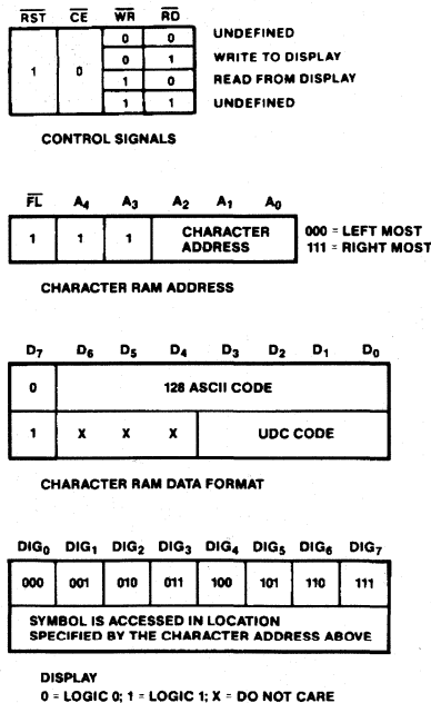
Figure 2. Logic Levels to Access the Character RAM.
