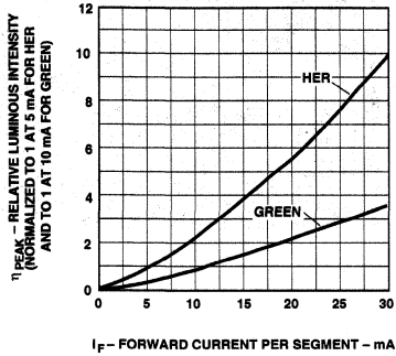
Figure 14. Relative Luminous Intensity vs. DC Forward Current.
