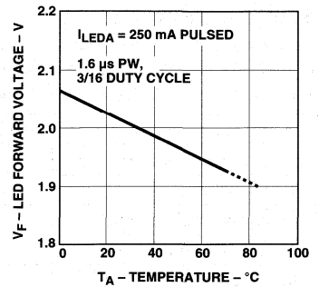
Figure 3. LED Forward Voltage vs. Temperature.
