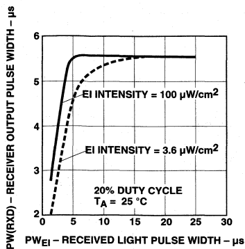
Figure 16. Receiver Output Pulse Width vs. Received Light Pulse Width.
