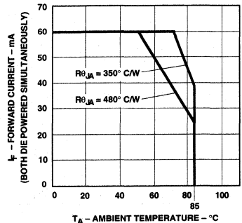
Figure 5b. Maximum Forward DC Current vs. Ambient Temperature, HLMP-V100.
