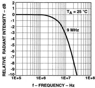
Figure 8. Relative Radiant Intensity vs. Frequency.
