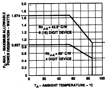
Figure 1. Maximum Allowable Power Dissipation vs. Ambient Temperature as a Function of Thermal Resistance IC Junction-to-Ambient, R_{\theta J-A} . Operation at 85^\circ\text{C} Assumes a Thermal Resistance for the Printed Circuit Board of R_{\theta PC-A} = 35^\circ\text{C/W} Per Device for the HCMS-270X, 17.5^\circ\text{C/W} Per Device for the HCMS-271X, and 17.5^\circ\text{C/W} Per Row for the HCMS-272X.
